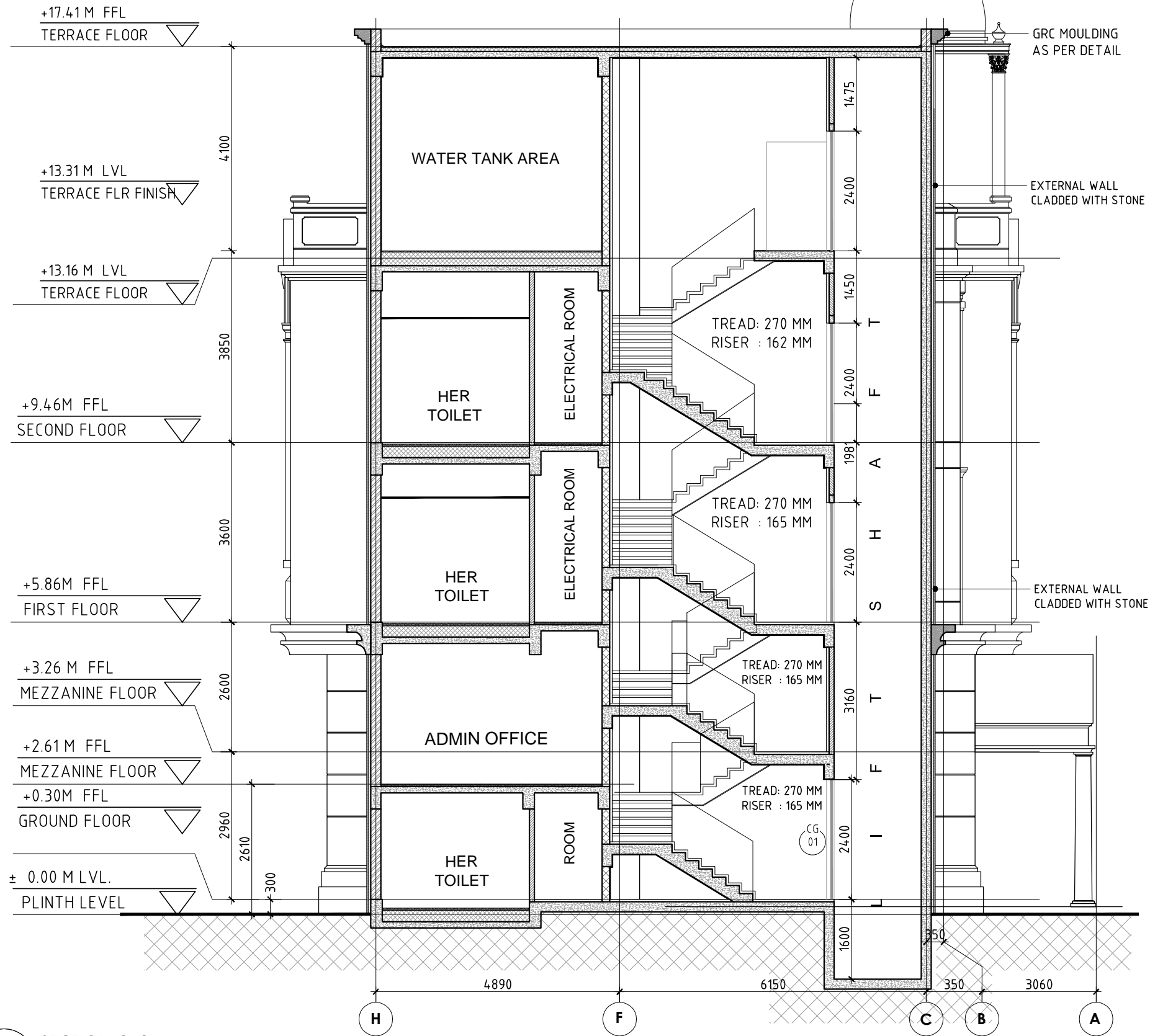
1 SECTION C-C SCALE 1:100
