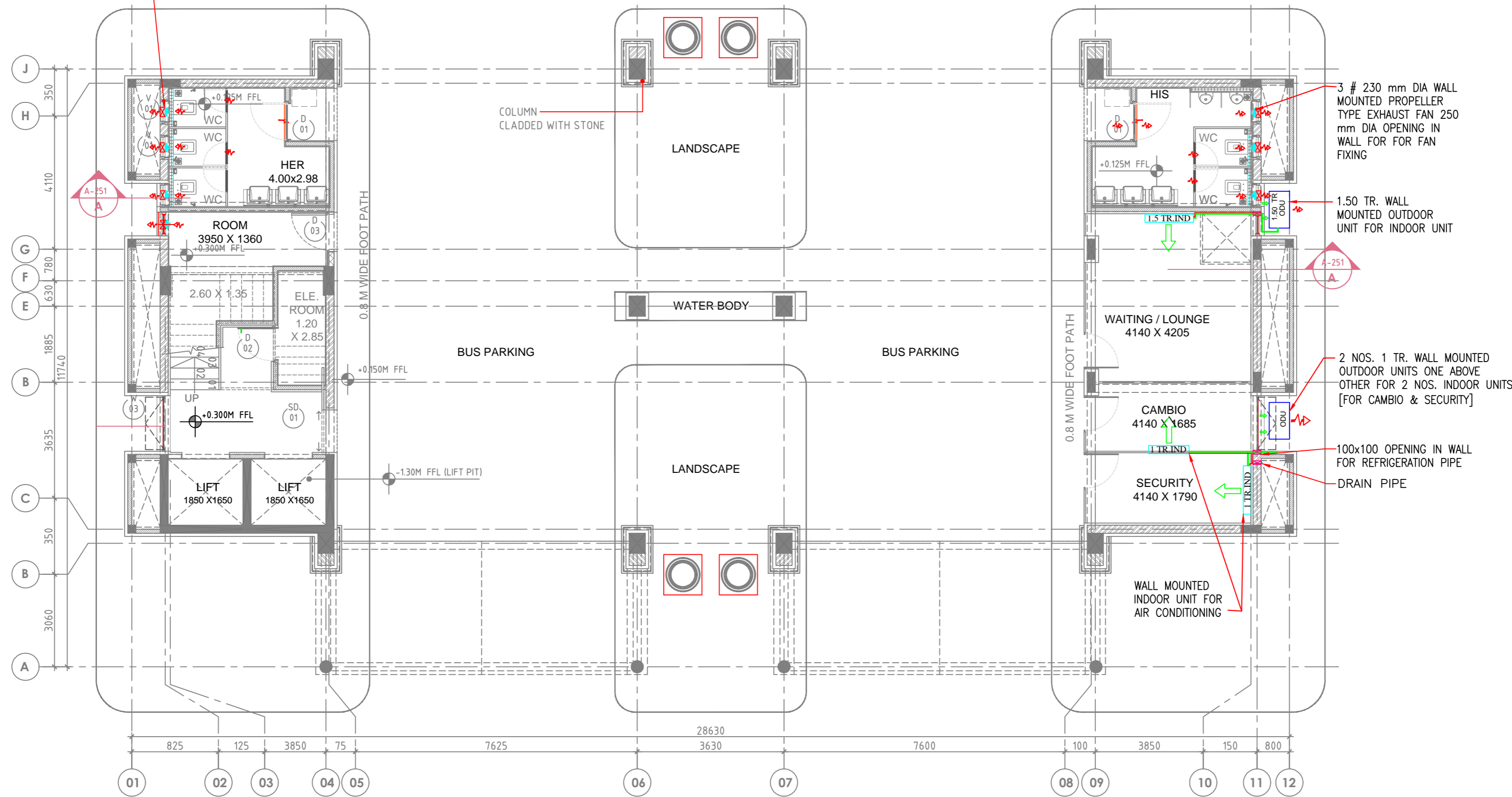
1 GROUND FLOOR PLAN SCALE 1:125
