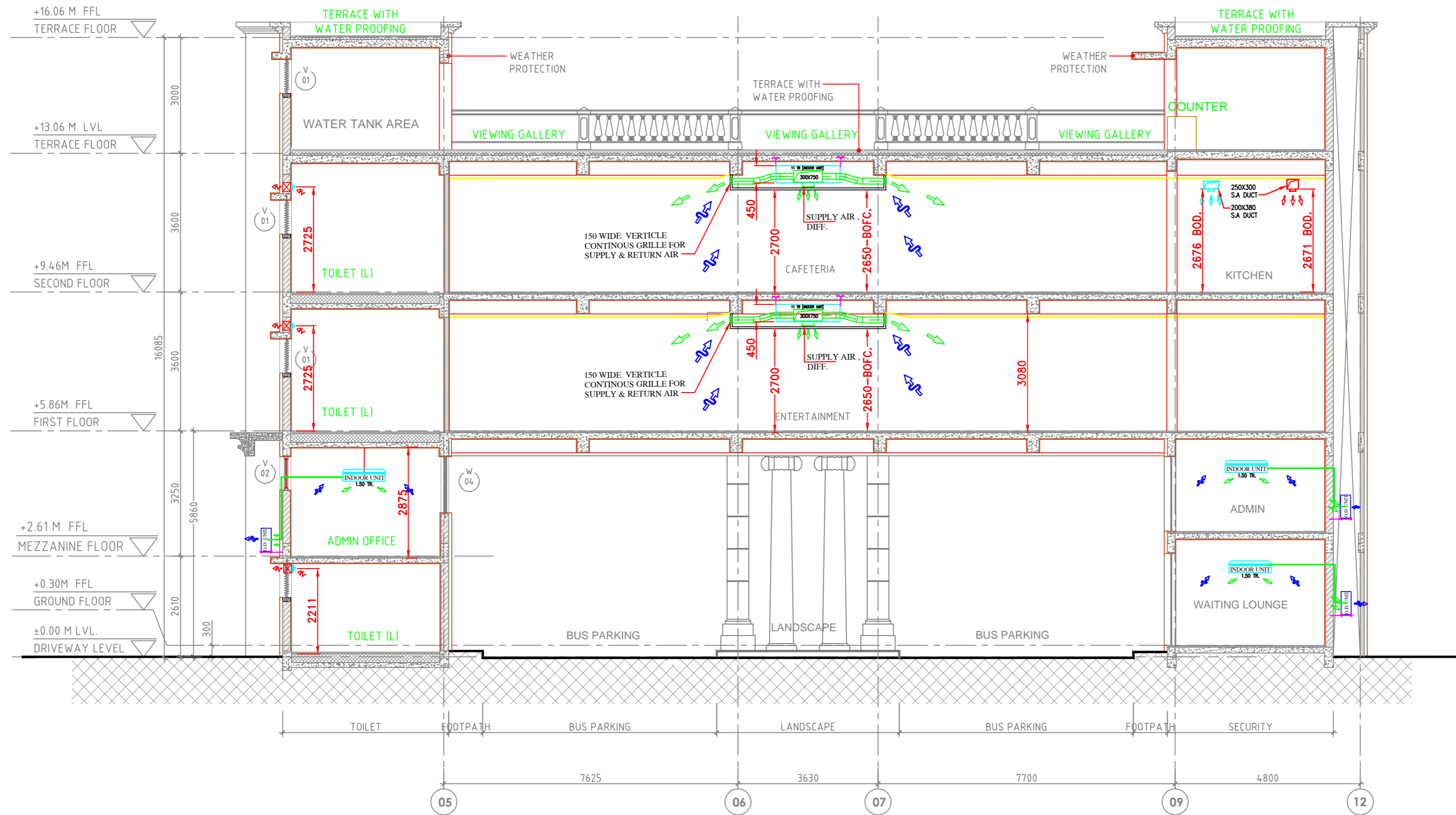
SECTION A - A SCALE 1:125
