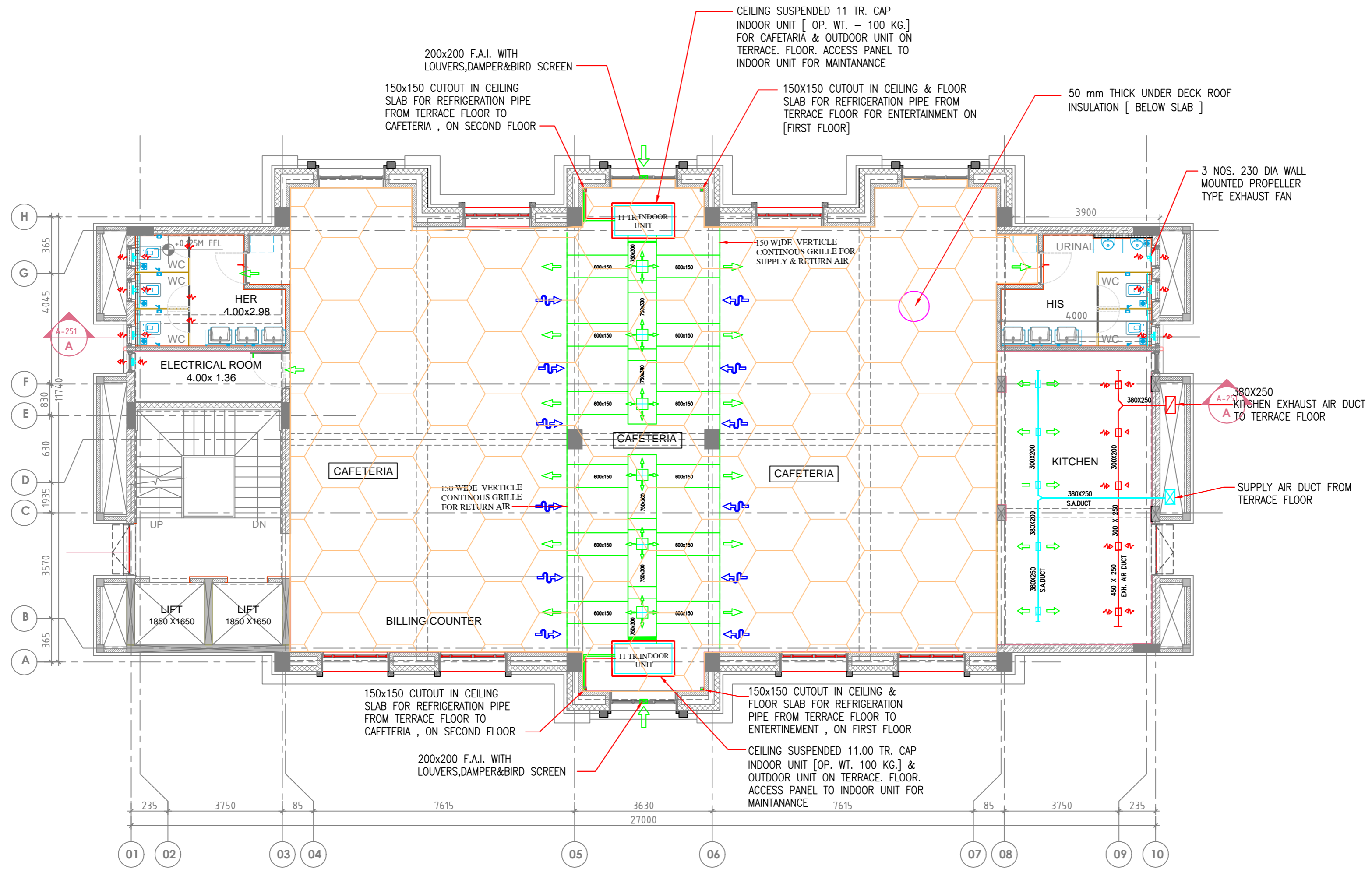
1 SECOND FLOOR PLAN SCALE 1:125
