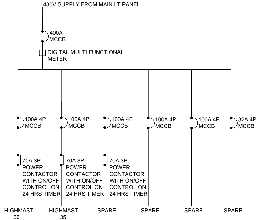
FEEDER PILLAR PANEL FOR T3 SHED
