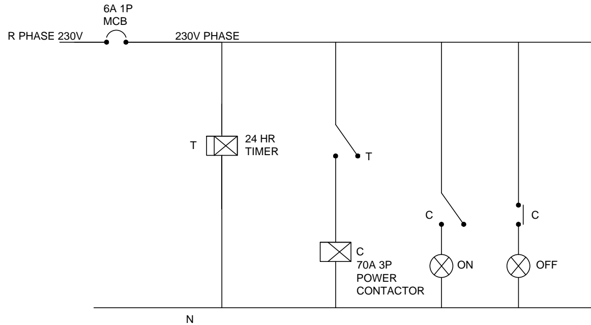
CONTROL CKT. FOR HIGHMAST LIGHTING
